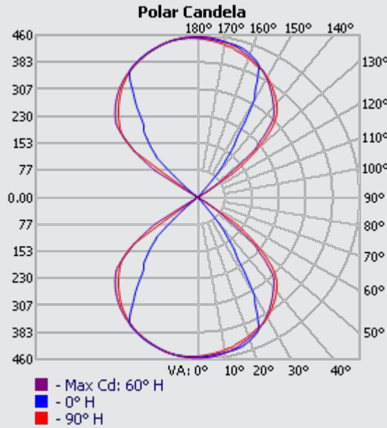
LUMINOUS INTENSITY DISTRIBUTION (20W 4K, FULL LIGHT)
