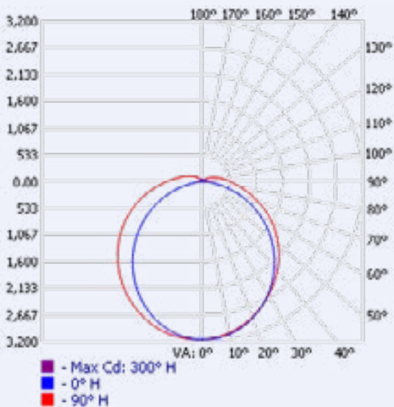
LUMINOUS INTENSITY DISTRIBUTION - R2 75W / 5K
