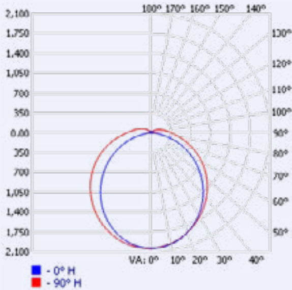
LUMINOUS INTENSITY DISTRIBUTION - R1 45W / 5K
